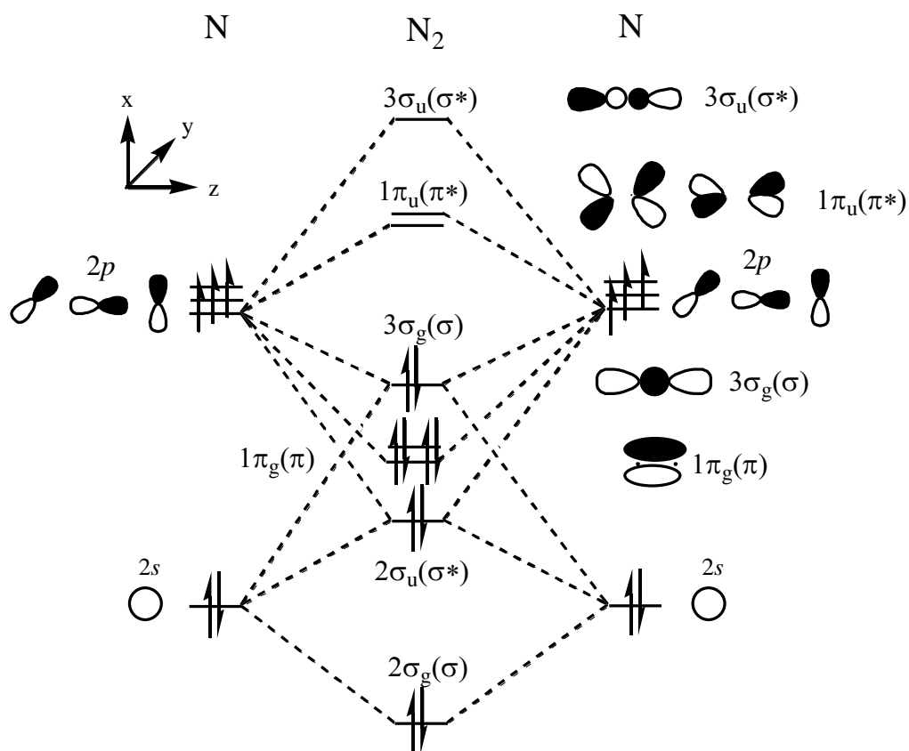
MO diagram of \text{N}_2
